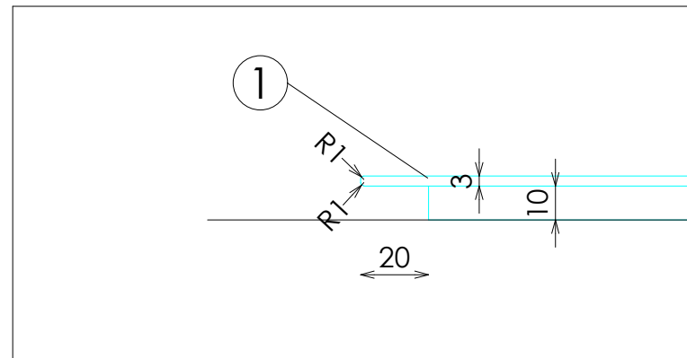
DETALLE TARIMA
