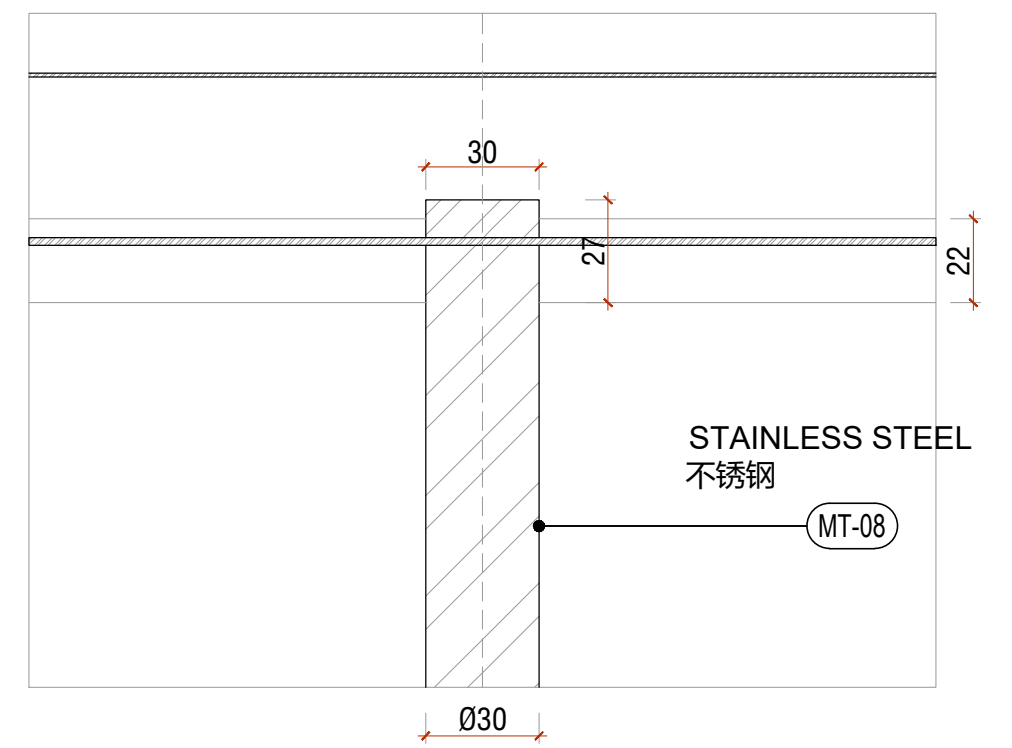
5 吊顶剖面节点 1:2 CEILING SECTION DETAIL
