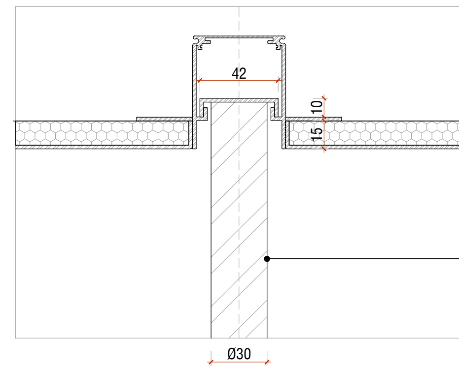
4 吊顶剖面节点 1:2 CEILING SECTION DETAIL
