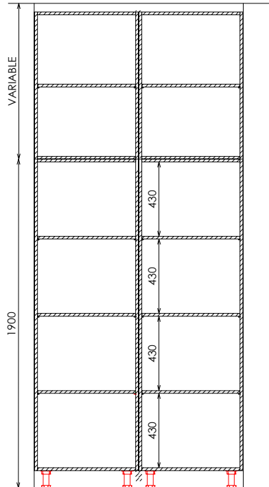
ALZADO INTERIOR
