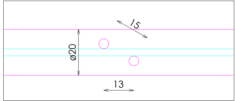
DETALLE TARIMA
