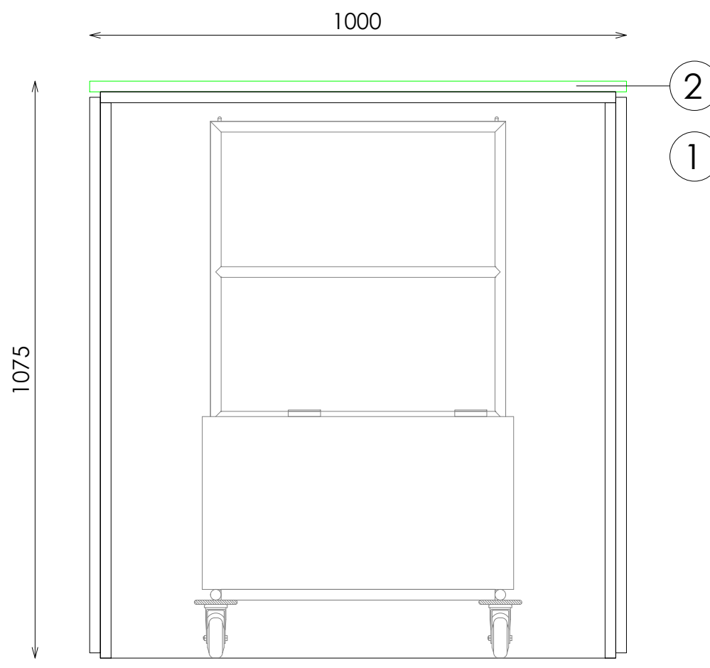
ALZADO INTERIOR
