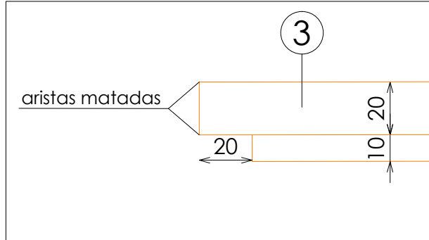
DETALLE TARIMA
