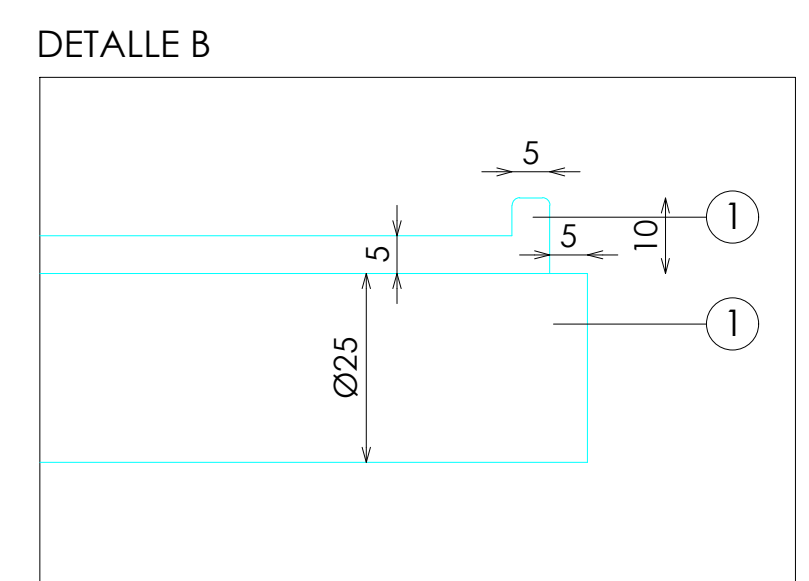
DETALLE BASE
