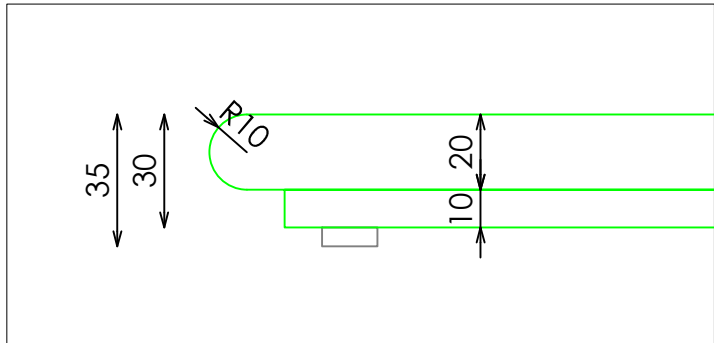
DETALLE TARIMA
