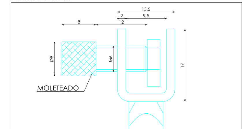
DETALLE CHAPA REMACHADA
