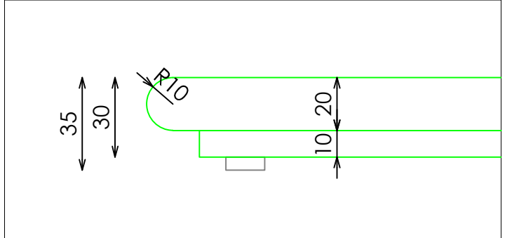
DETALLE TARIMA
