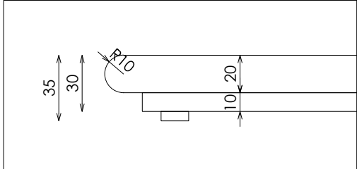
DETALLE TARIMA
