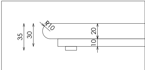
DETALLE TARIMA
