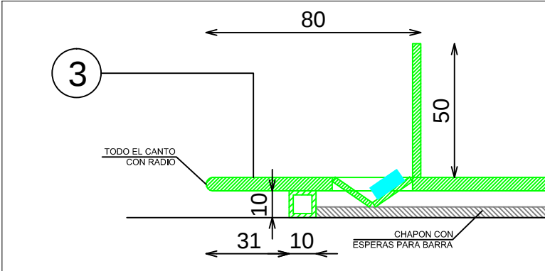
DETALLE BASE
