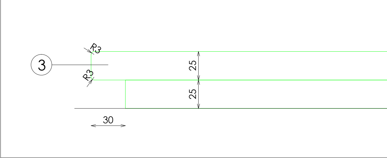
DETALLE BASE
