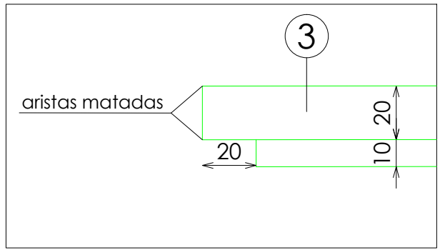
DETALLE TARIMA
