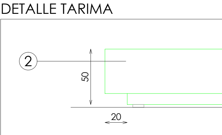
DETALLE TARIMA
