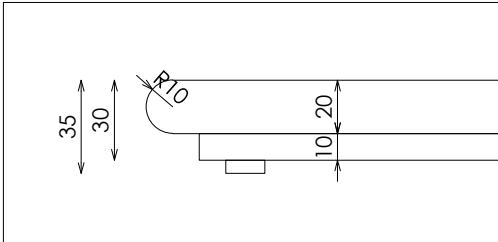
DETALLE TARIMA
