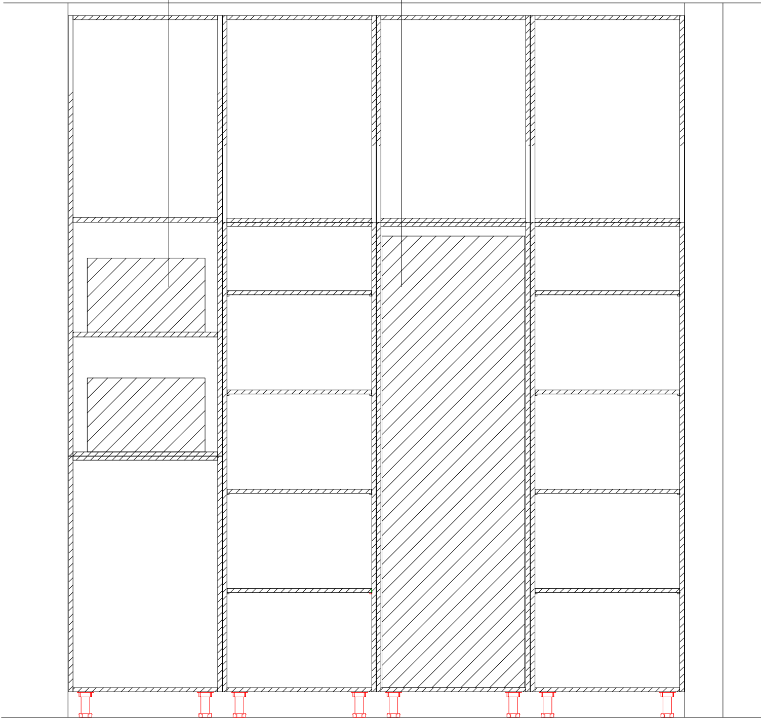
ALZADO INTERIOR
