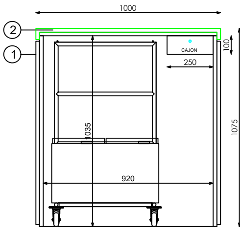
ALZADO INTERIOR
