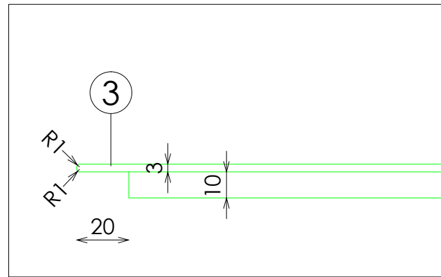
DETALLE TARIMA
