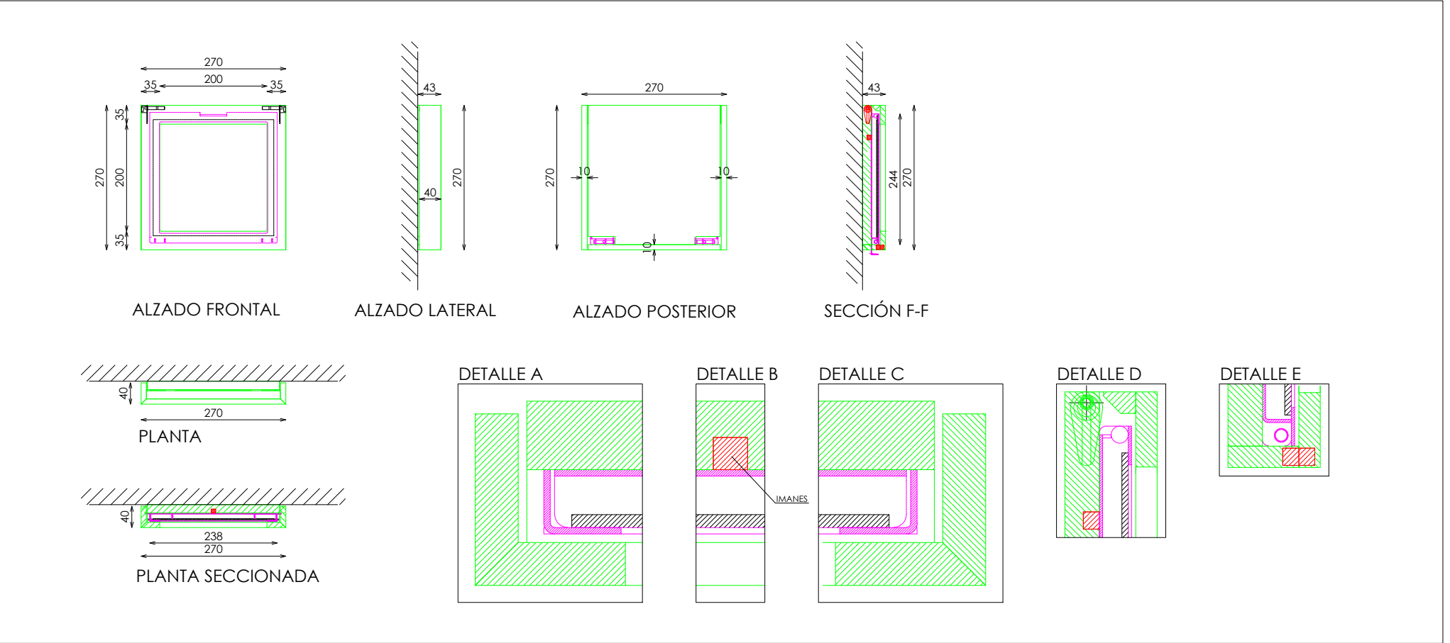
DETALLE MARCO INTERIOR
