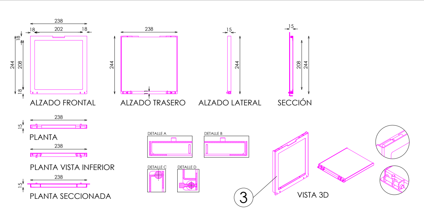
DETALLE MARCO INTERIOR
