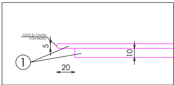
DETALLE TARIMA
