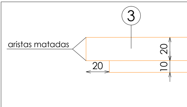
DETALLE TARIMA
