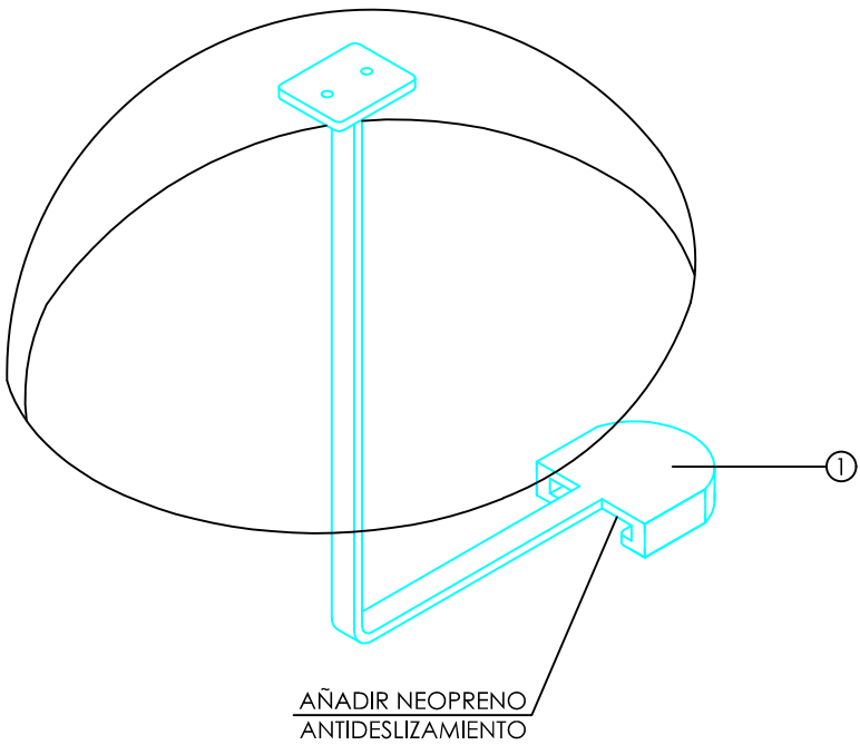
VISTA 3D
