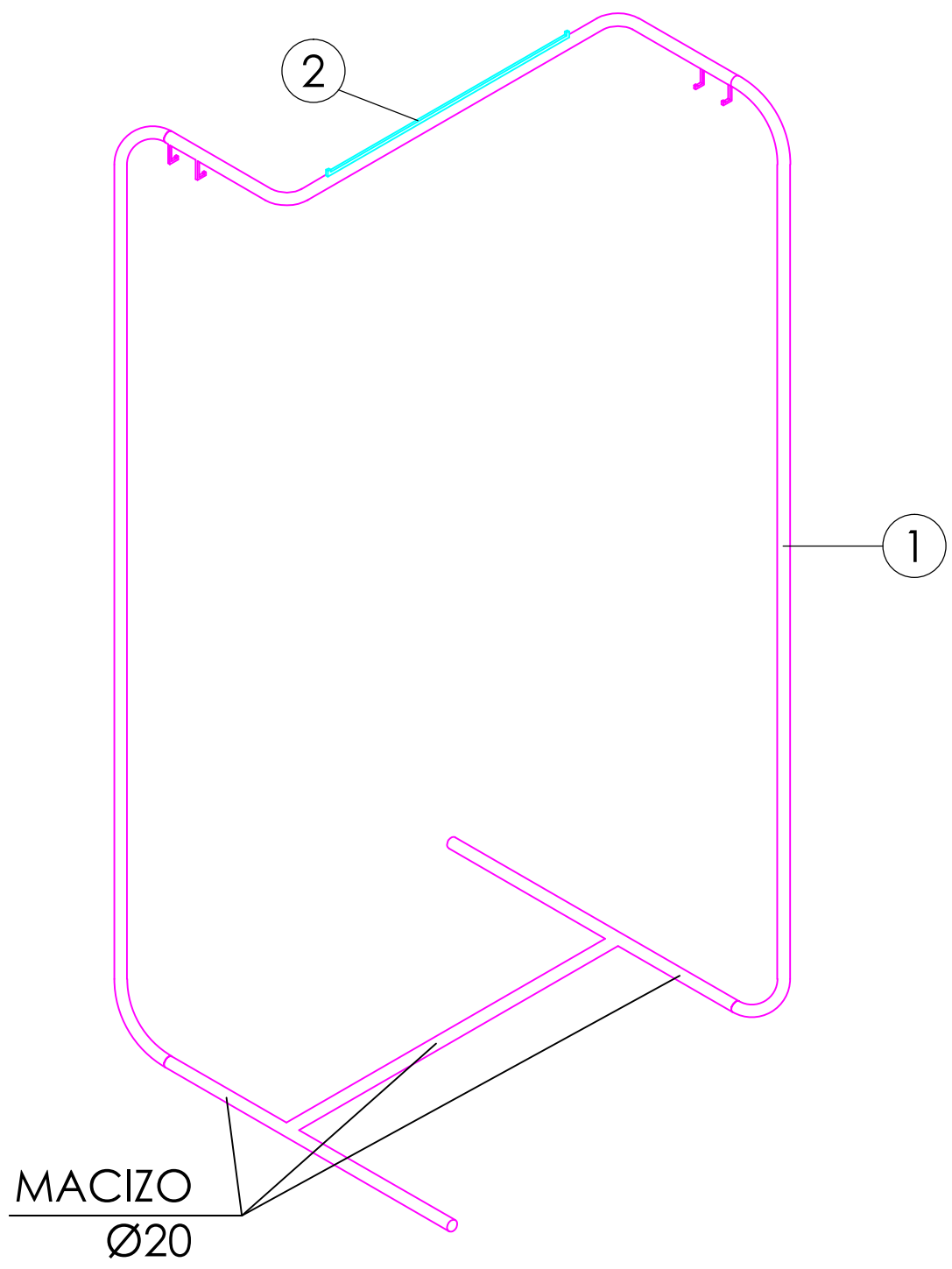
VISTA 3D
