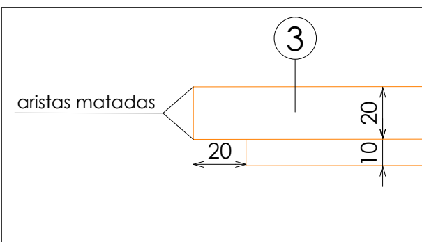
DETALLE TARIMA
