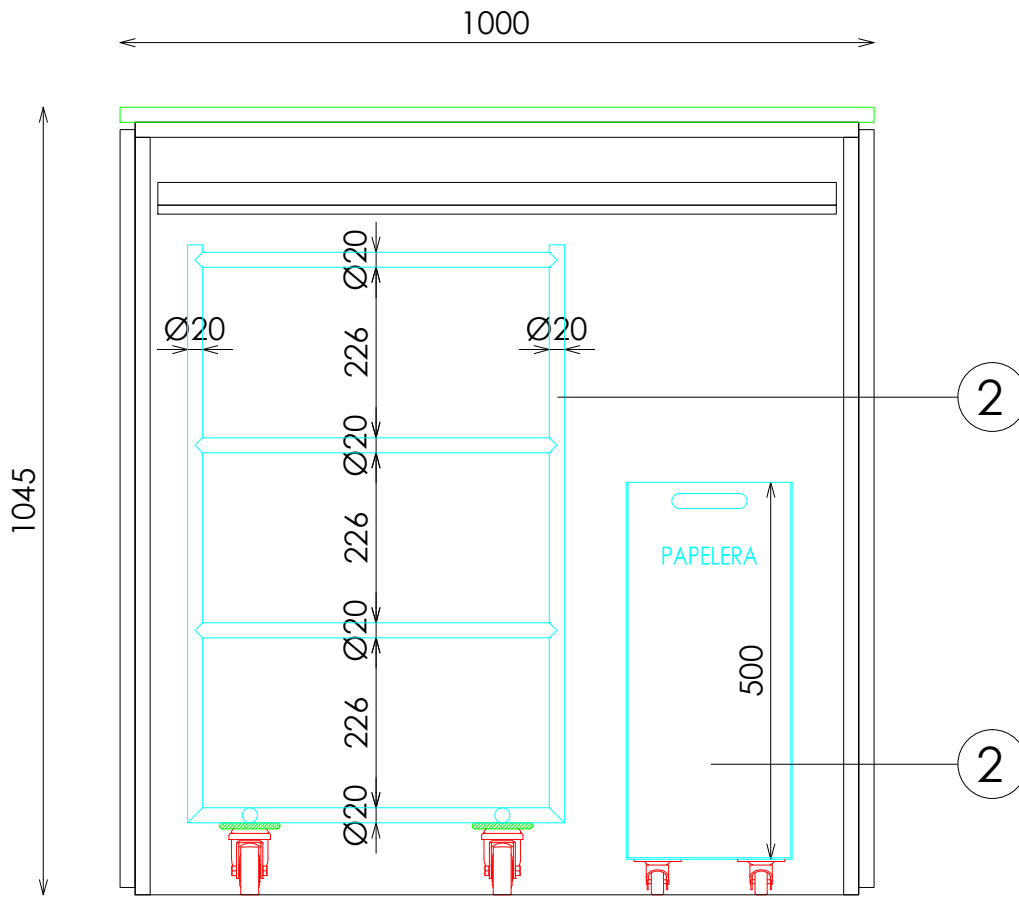
ALZADO INTERIOR
