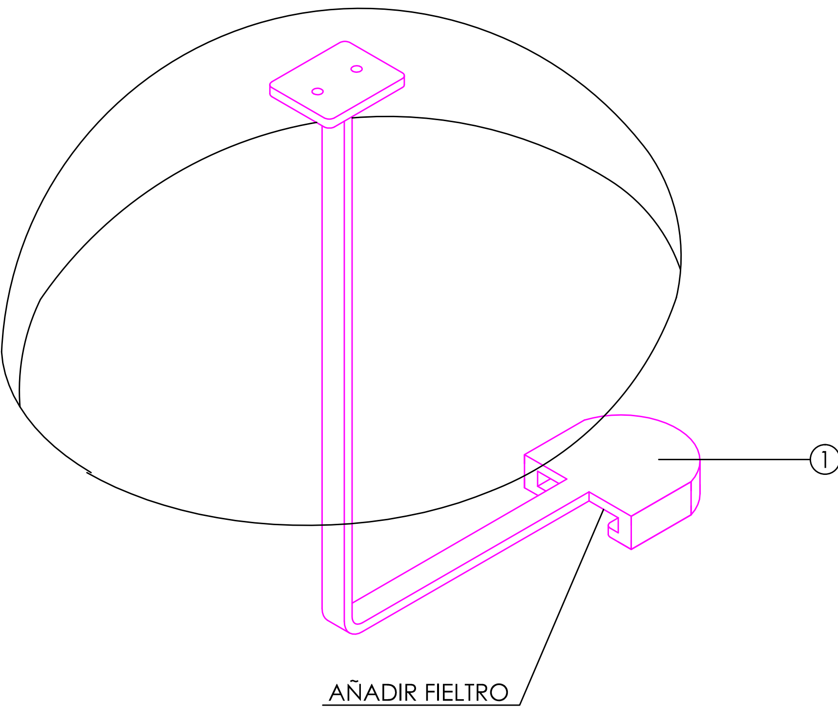
VISTA 3D
