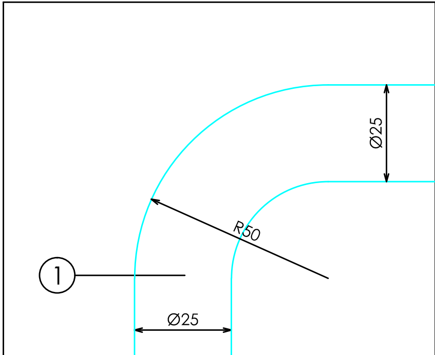
DETALLE UNION INTERMEDIA BARRAS VERTICALES
