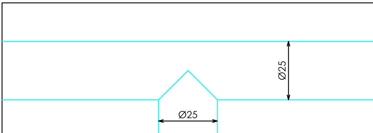
DETALLE UNION INTERMEDIA BARRAS VERTICALES
