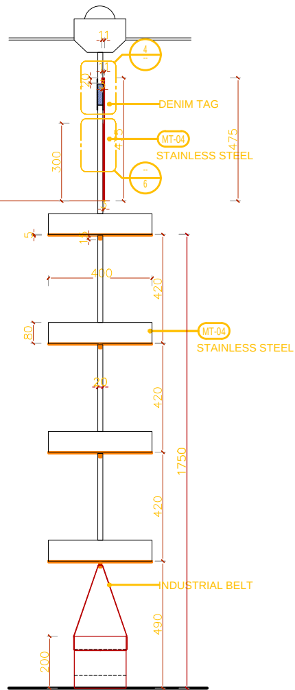
2 1:10 SECTION
