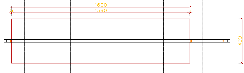
3 1:10 SECTION PLAN
