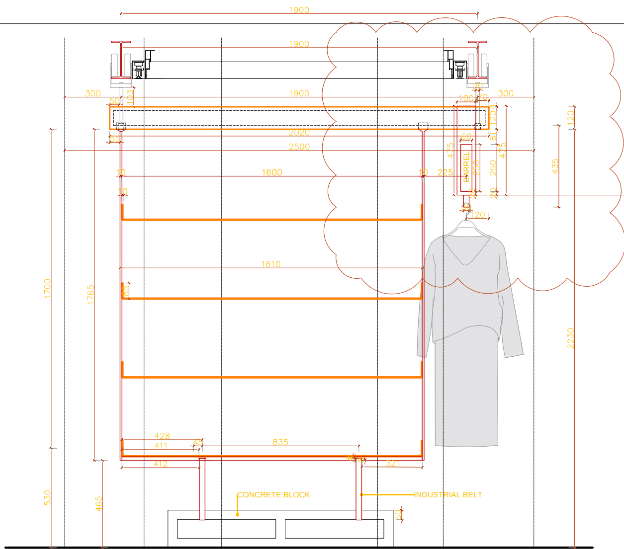
1 1:10 FRONT ELEVATION
