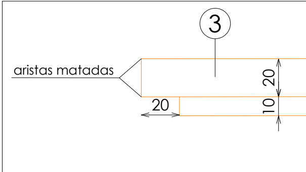
DETALLE TARIMA
