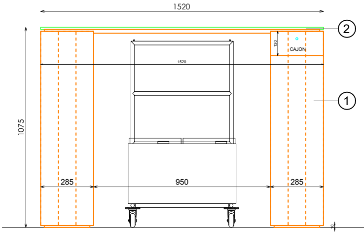
ALZADO INTERIOR
