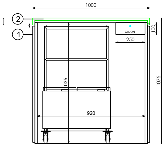
ALZADO INTERIOR
